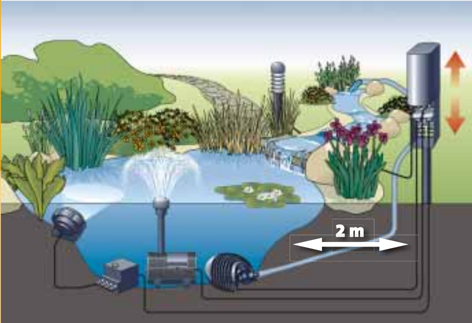
Schematic representation: Connection possibilities with the InScenio OASE garden outlets
