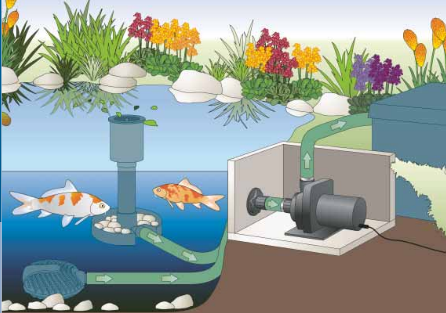
Schematic representation: Dry installation for Filter and Watercourse pump Aquamax Dry 14000 (PRO) with concurrent operation of skimmer and satellite filter
